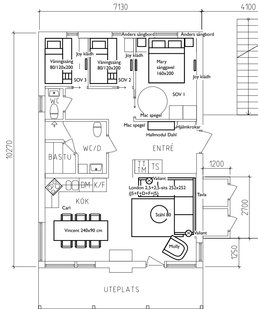
BOTTENPLAN
